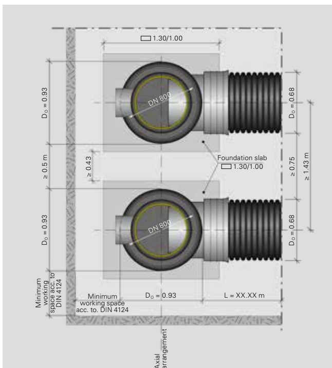
Axial arrangement
