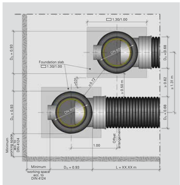
Offset arrangement
